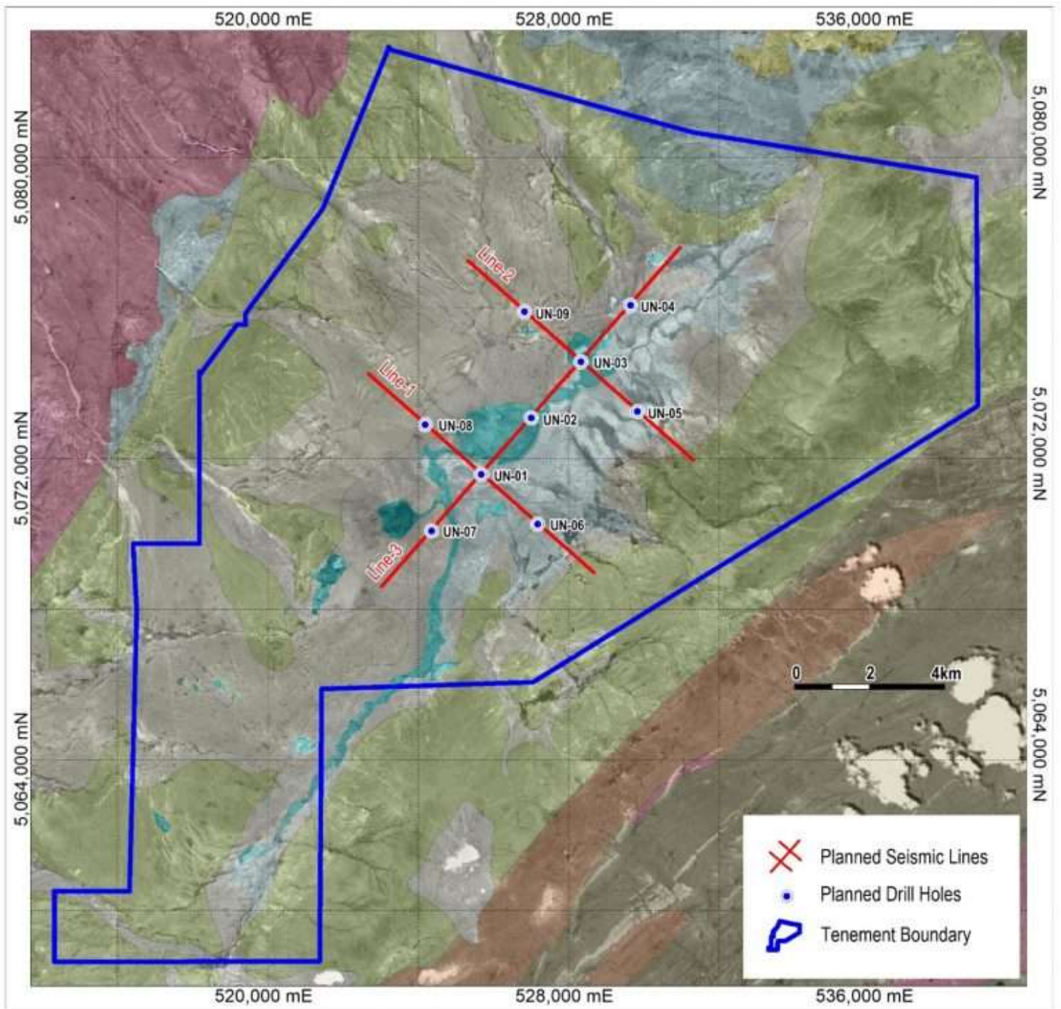
Proposed Shallow Refraction Seismic Survey lines and drill hole location at Urgakh Naran project.
